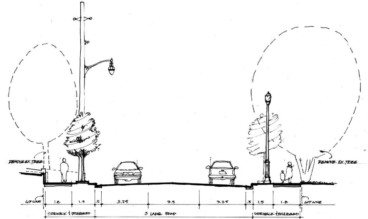
3 LANE WIDENING AT HUNTER STREET LOOKING SOUTH ON WARD ST.
