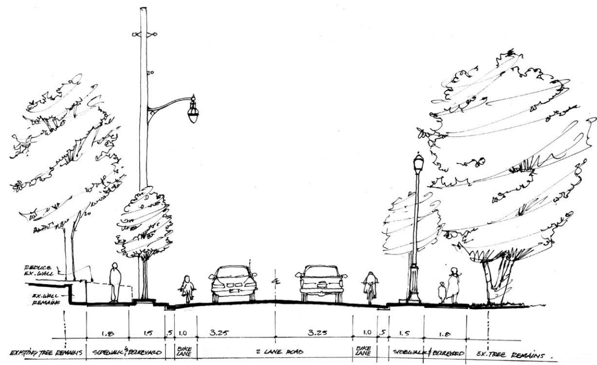
EXISTING ROAD WIDTH WITH NEW SIDEWALKS & BOULEVARDS & CURBS. LOOKING SOUTH ON WARD STREET AT HUNTER.
