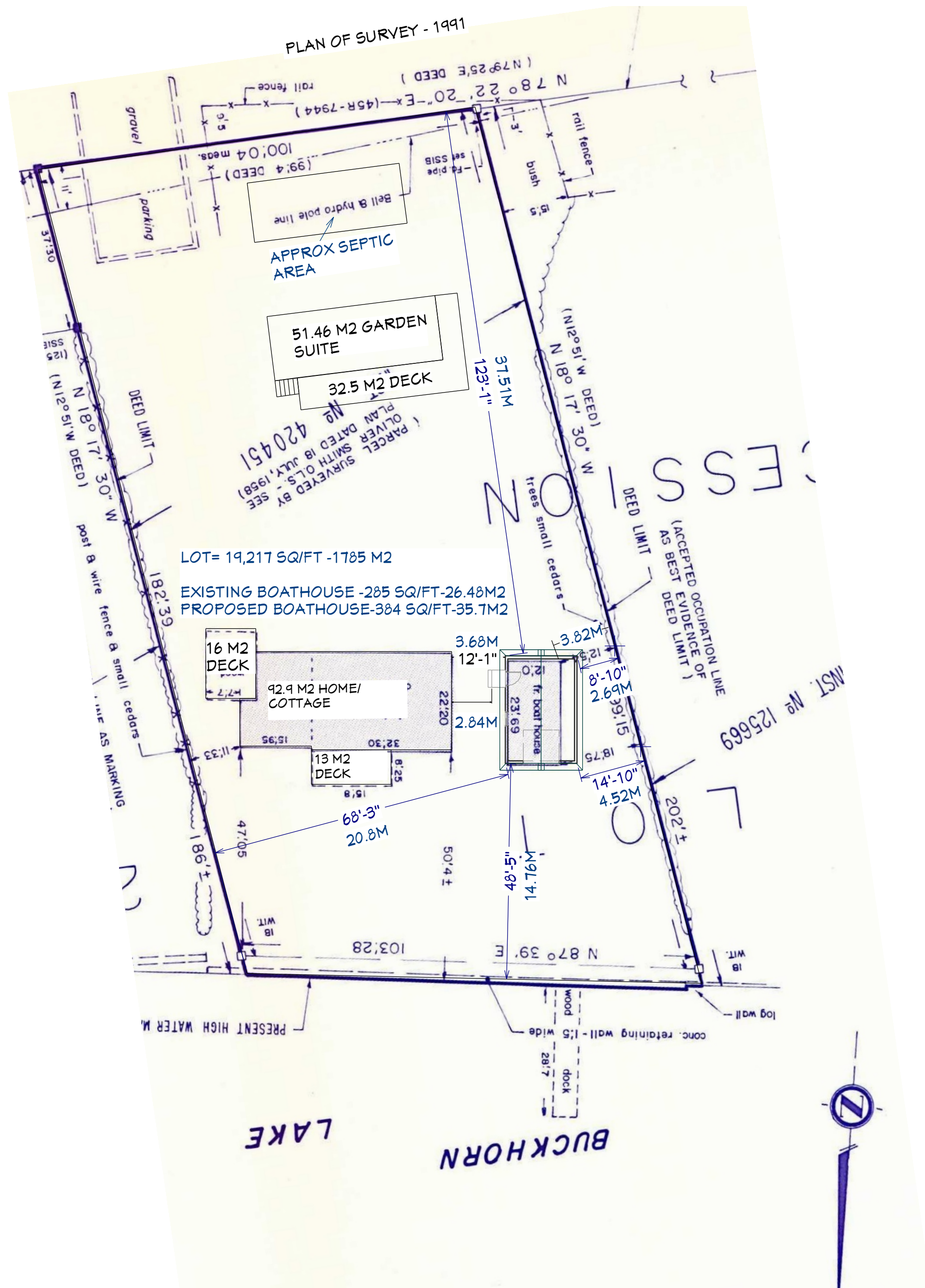
Plot Plan View
